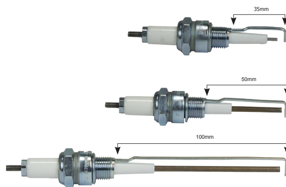
The 35 mm, 50 mm and 100 mm spark plugs
