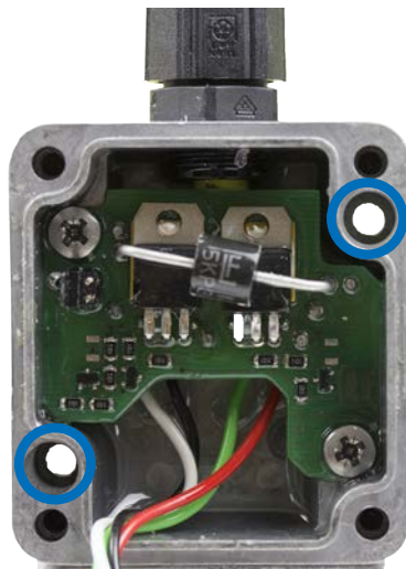
Mounting Holes
