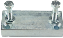
Fig. 4 - Mounting block for pivot joint
