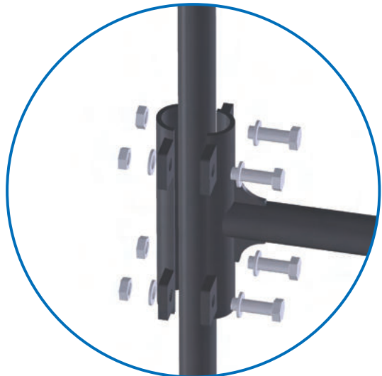
Figure 32: The mounting tube is imounted with four bolts
