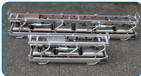
Fig. 1 - Joint Heater, 12/24V, 3, 6 burner (S-50464, S-50418)
