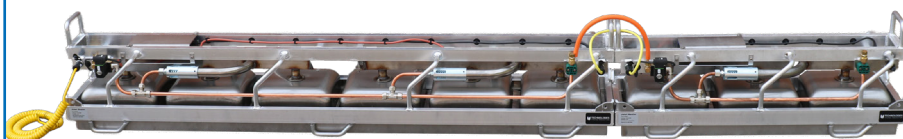
Fig. 2 - Joint Heater Extension, Connection of 6 burner and 3 burner version for a 9 burner Joint Heater
