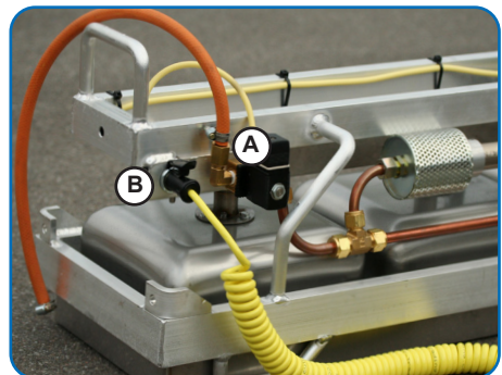
Fig. 5 - Joint Heater Power supply
