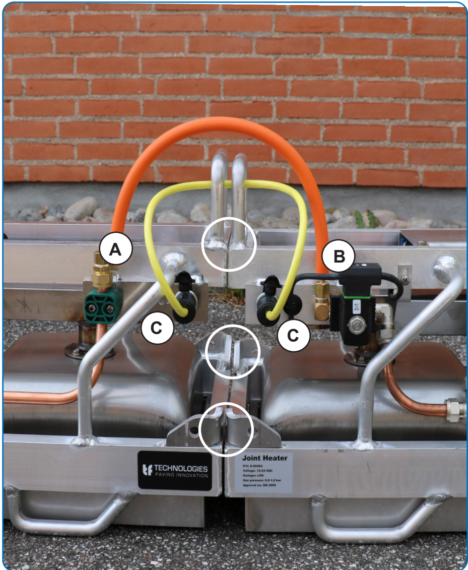
Fig. 6 - Joint Heater Udgrading, Connection of 6 burner and 3 burner version for a 9 burner Joint Heater
