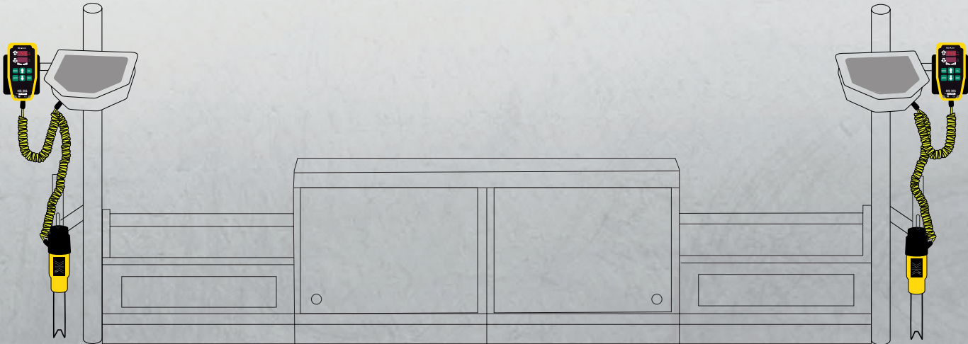
HS301 Double Grade Control Kit with G221 Single-Sonic sensors as set up on the asphalt paver. Sensor and controller connect to the 10-pin plug of the asphalt paver with a V-Cable in each side of the screed.
