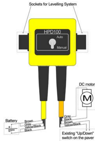
Figure 1 - HPD100 construction
