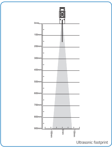
G221 Sonic Sensor
