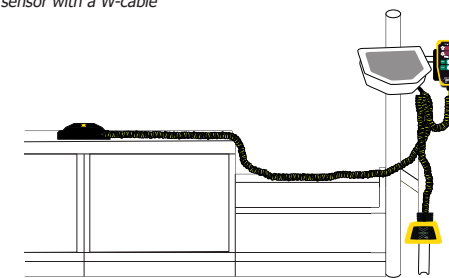
Connecting the HS301, G224 grade sensor and S298 slope sensor with a W-cable
