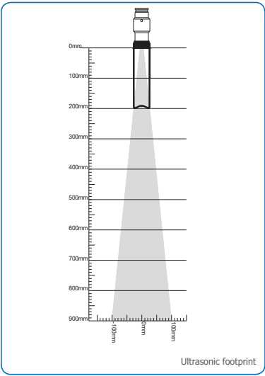
G220 Sonic Sensor
