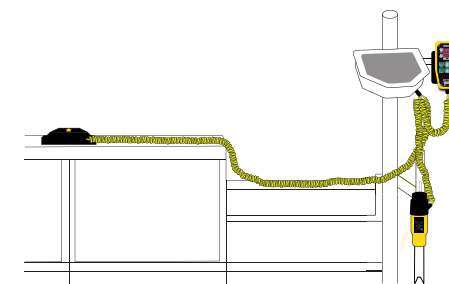
Connecting the HS301, G221 grade sensor and S298 slope sensor with a W-cable
